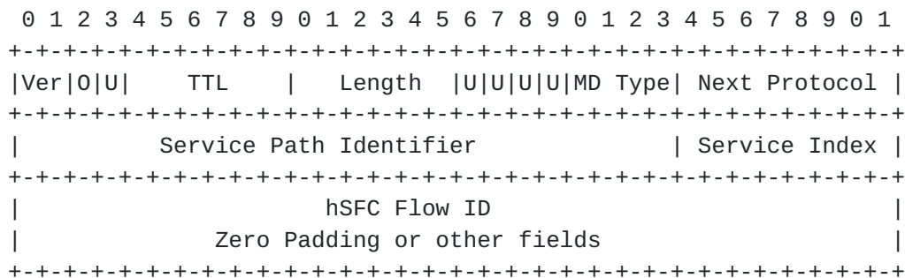
Figure 4: Storing hSFC Flow ID in lower-level NSH Fixed-Length Context Header ( [RFC8300] , Section 2.4 )
