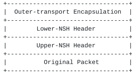
Figure 3: Encapsulation of NSH within NSH
