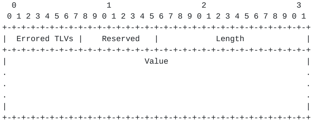
Figure 5: Errored TLVs TLV
