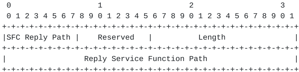
Figure 7: SFC Reply TLV Format
