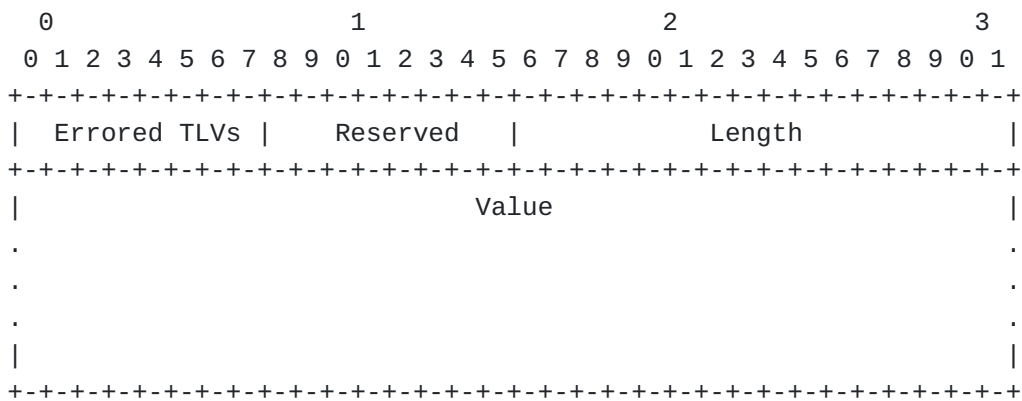
Figure 6: Errored TLVs TLV
