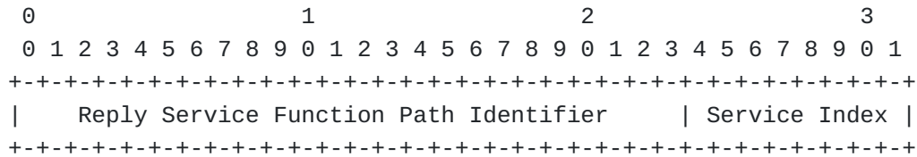
Figure 8: Reply Service Function Path Field Format
