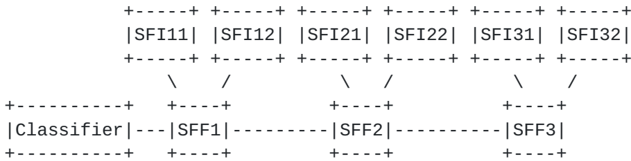
Figure 1: An Example of SFC Data Plane Architecture
