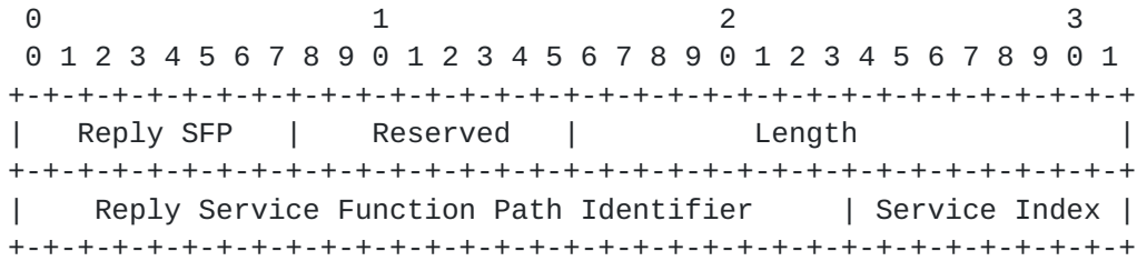
Figure 8: SFC Reply TLV Format
