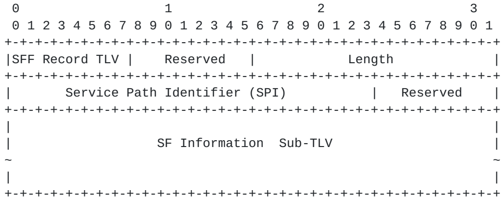
Figure 9: SFF Information Record TLV
