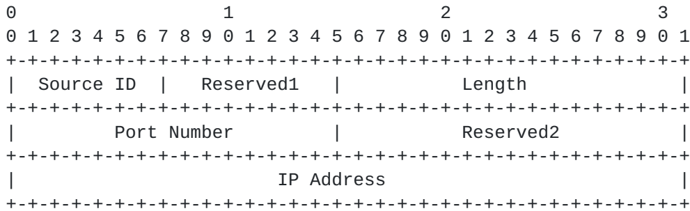
Figure 5: SFC Source TLV
