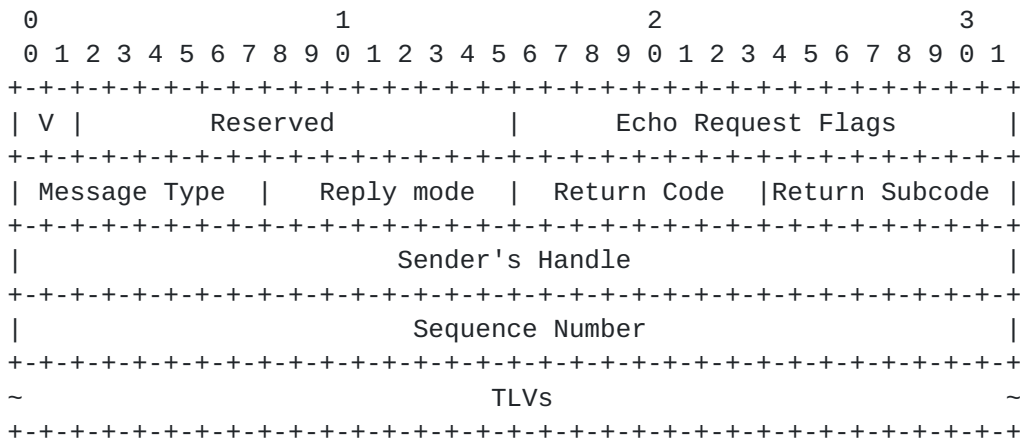
Figure 3: SFC Echo Request/Reply Format
