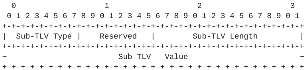
Figure 7: Not Understood or Failed TLV as Sub-TLV
