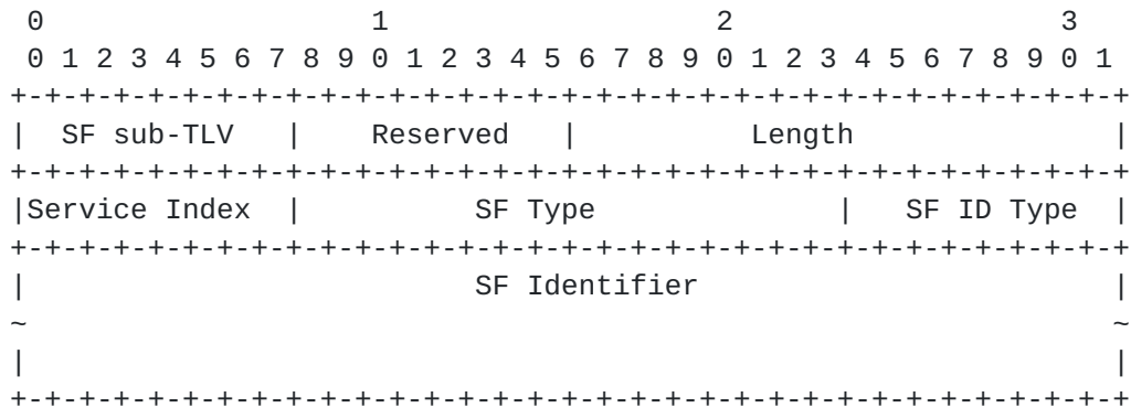
Figure 10: Service Function Information Sub-TLV
