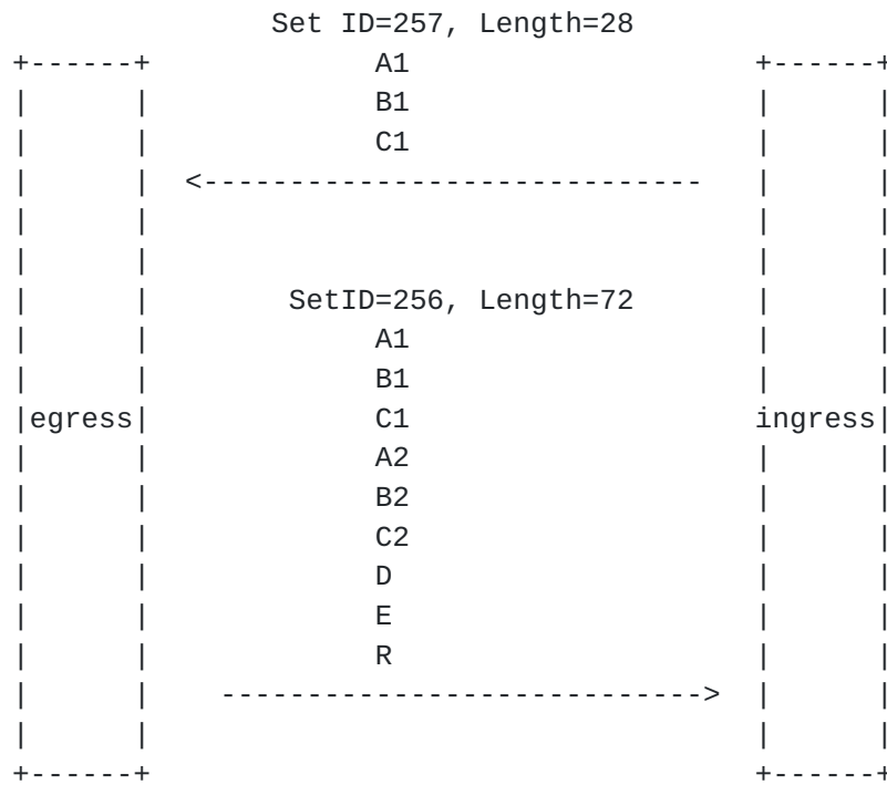
Figure 10. Messages Between Ingress and Egress
