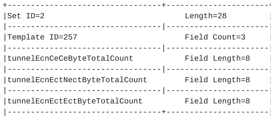
Figure 8. Template Record Sent From Ingress to Egress
