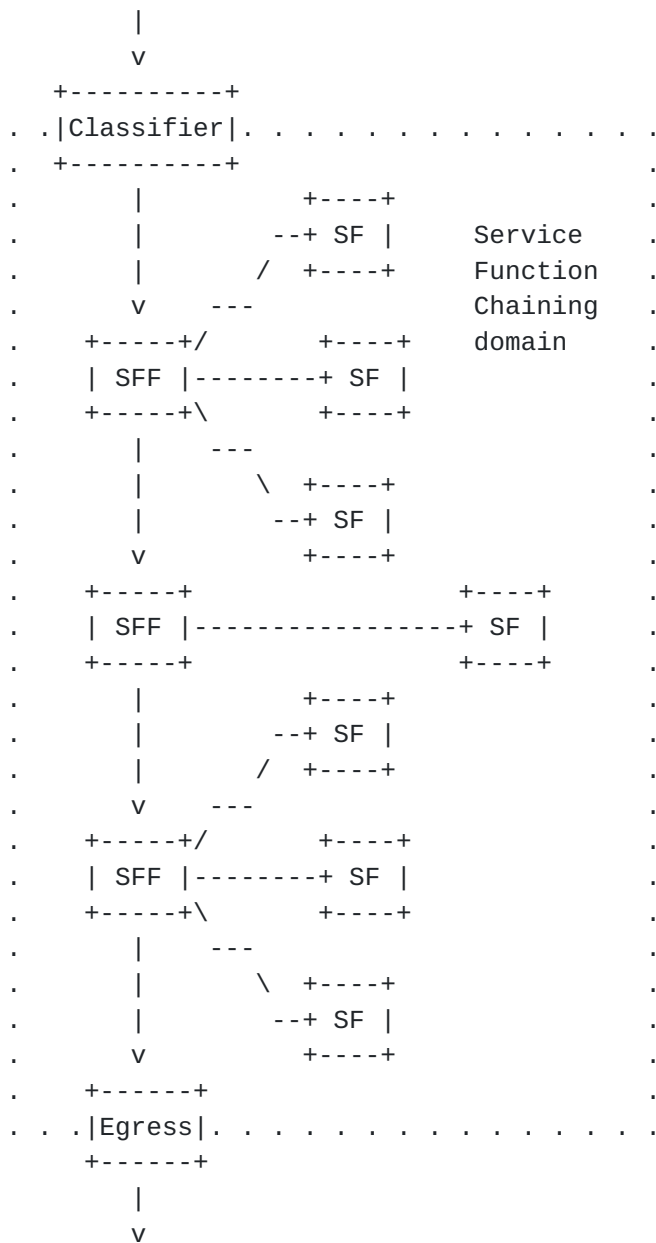
Figure 1. Example SFC Forwarding Nodes Path
