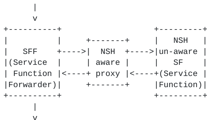
Figure 6. Proxy for NSH Un-aware SFF
