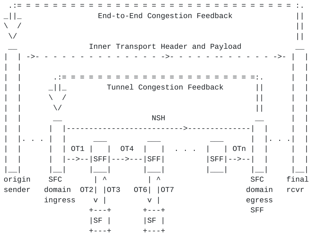
Figure 2. Congestion Feedback across an SFC enabled Domain
