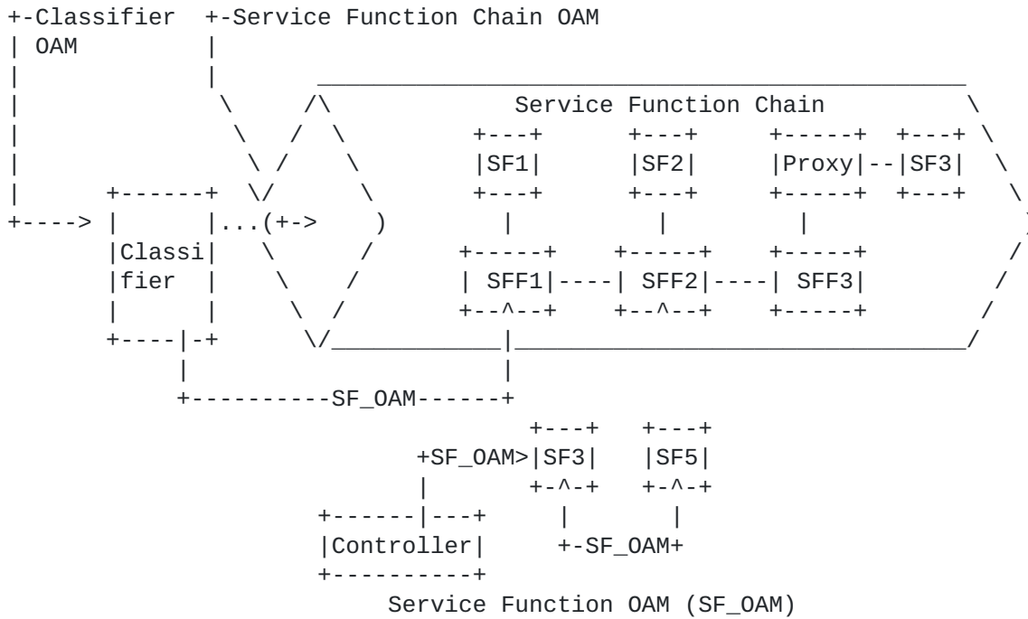
Figure 2: SFC OAM for Three Components
