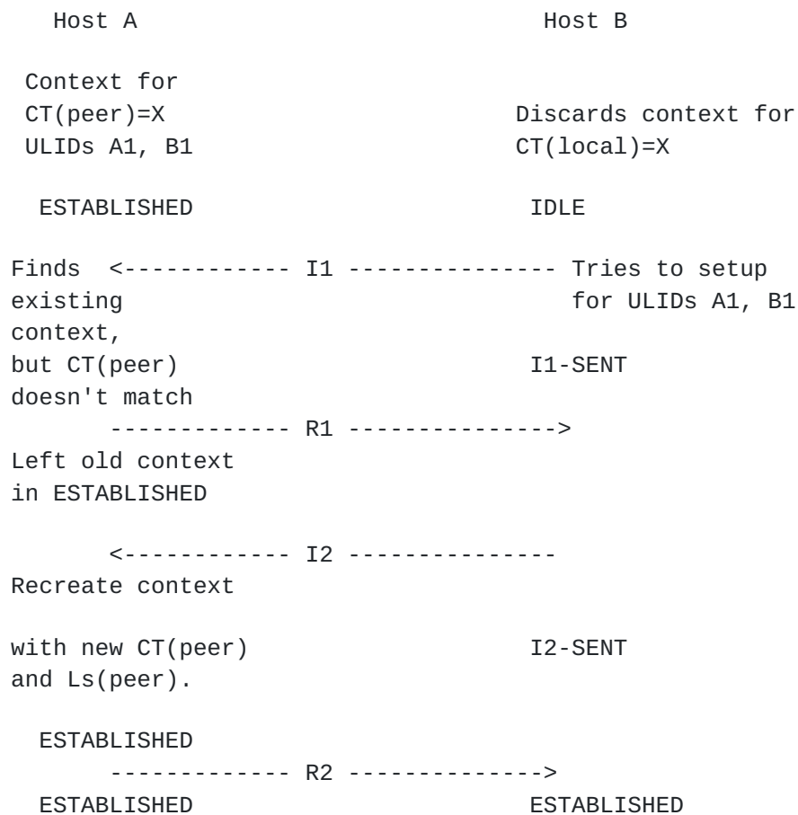
Figure 7: Context loss at sender
