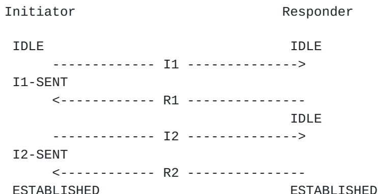
Figure 3: Normal context establishment
