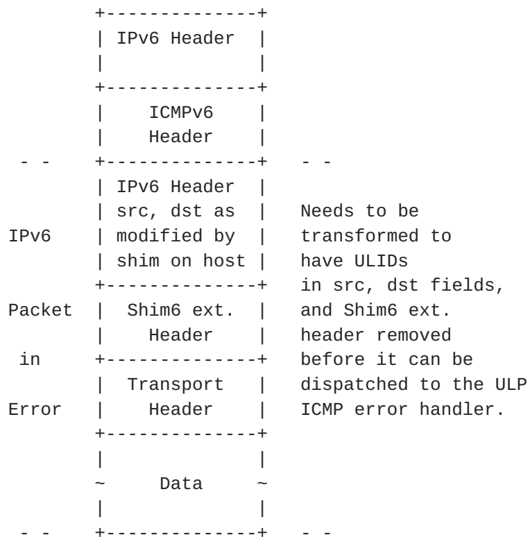
Figure 9: ICMP error handling with payload extension header
