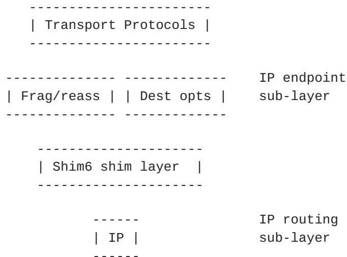
Figure 1: Protocol stack
