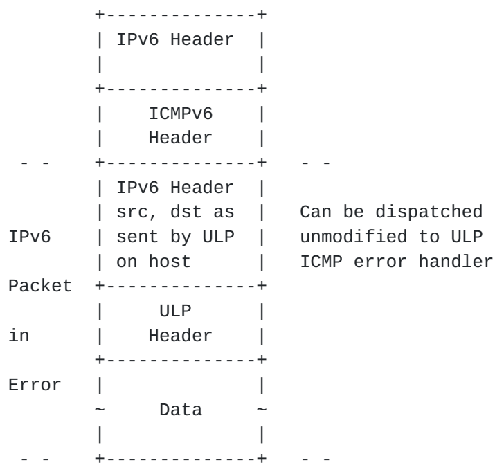
Figure 8: ICMP error handling without payload extension header
