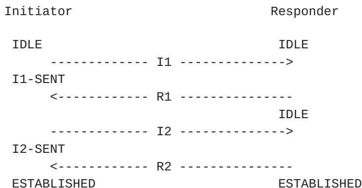
Figure 3: Normal context establishment
