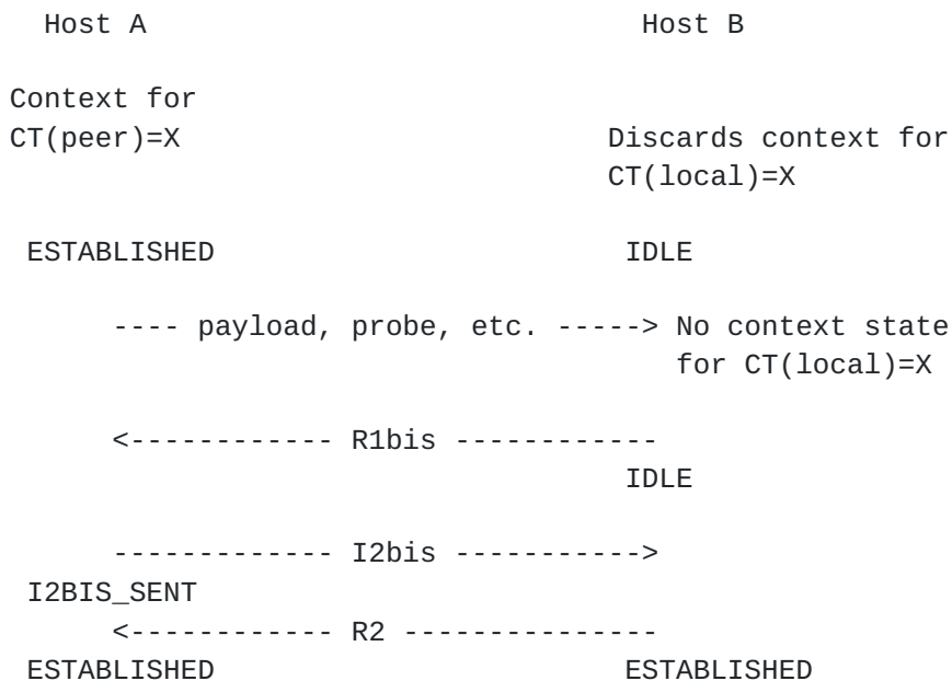
Figure 6: Context loss at receiver
