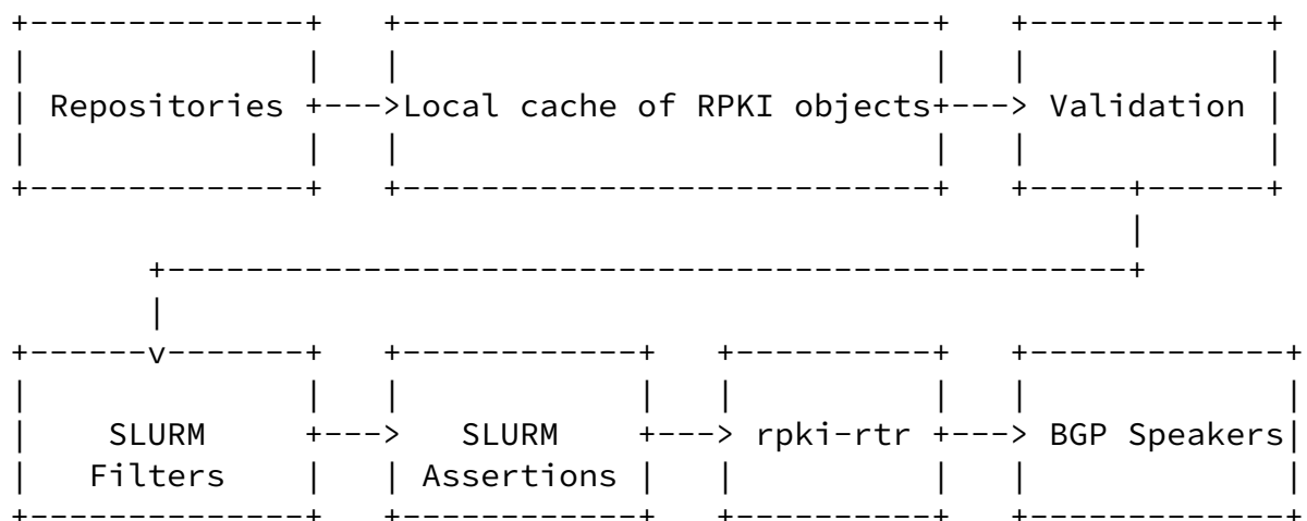
Figure 1: SLURM's Position in the RP Stack
