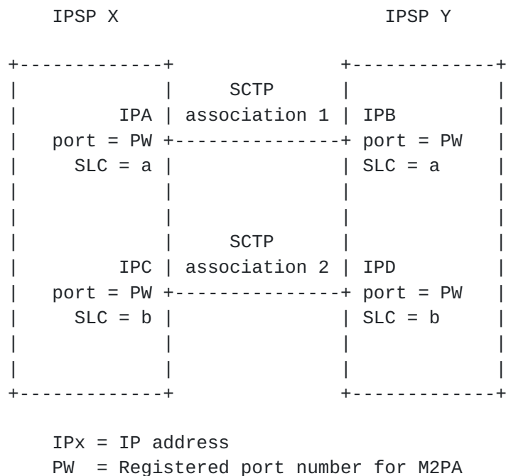
Figure 8. Two IPSPs with Two IP Addresses Each
