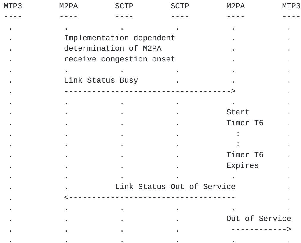
Figure 18. Example: Level 2 Flow Control - Timer T6 Expires
