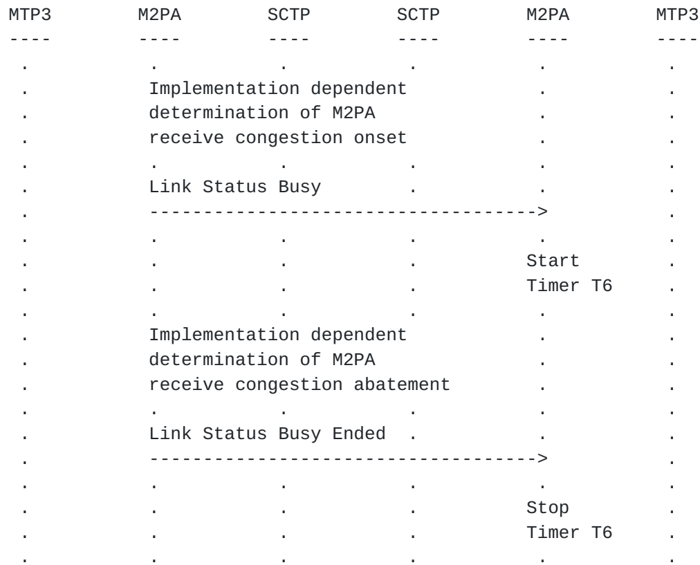
Figure 17. Example: Level 2 Flow Control - Congestion Ceases
