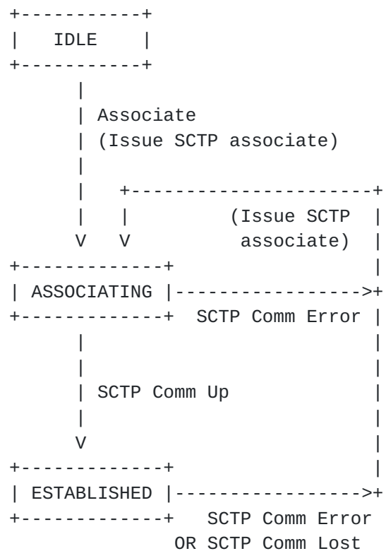
Figure 7. M2PA Association State Transition Diagram
