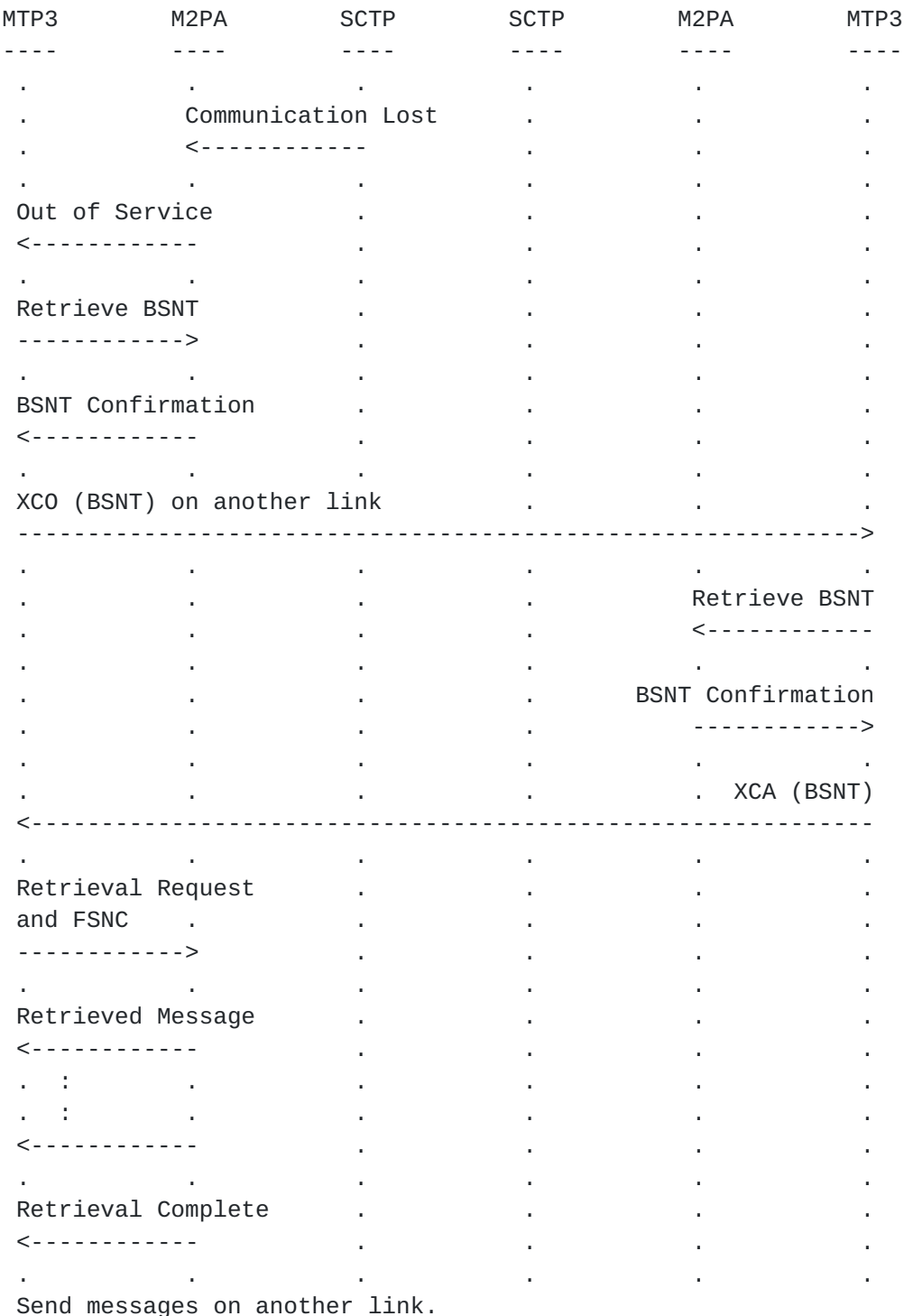
Figure 21. Example: Link Changeover
