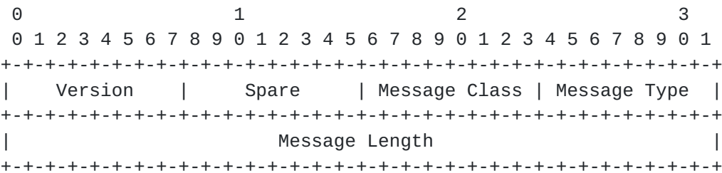
Figure 5. Common Message Header
