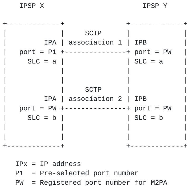
Figure 10. Multiple Associations Between Two IP Addresses
