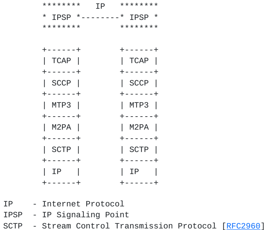
Figure 1. M2PA Symmetrical Peer-to-Peer Architecture
