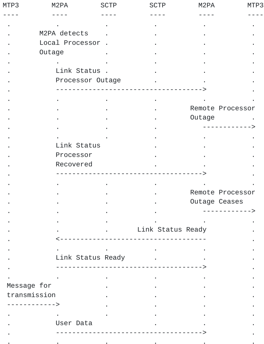
Figure 15. Example: Link Status Message - Processor Outage
