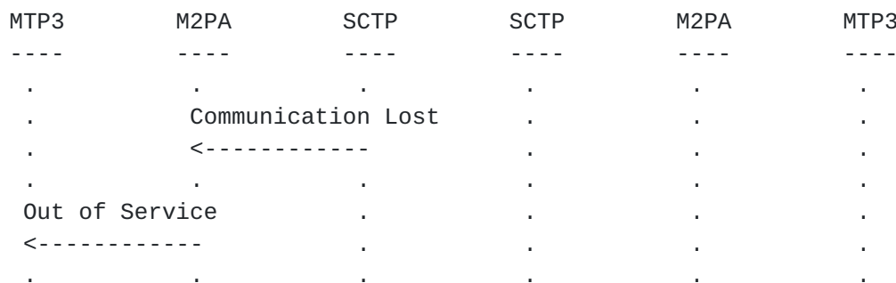
Figure 14. Example: Link Status Indication
