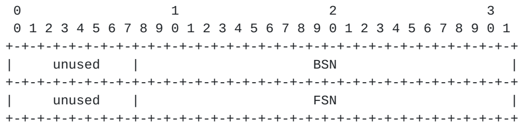
Figure 6. M2PA-specific Message Header
