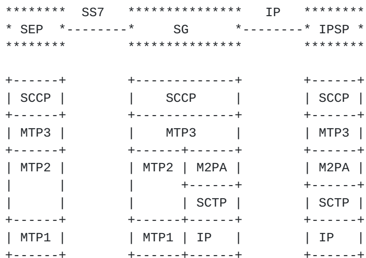
Figure 3. M2PA in IP Signaling Gateway
