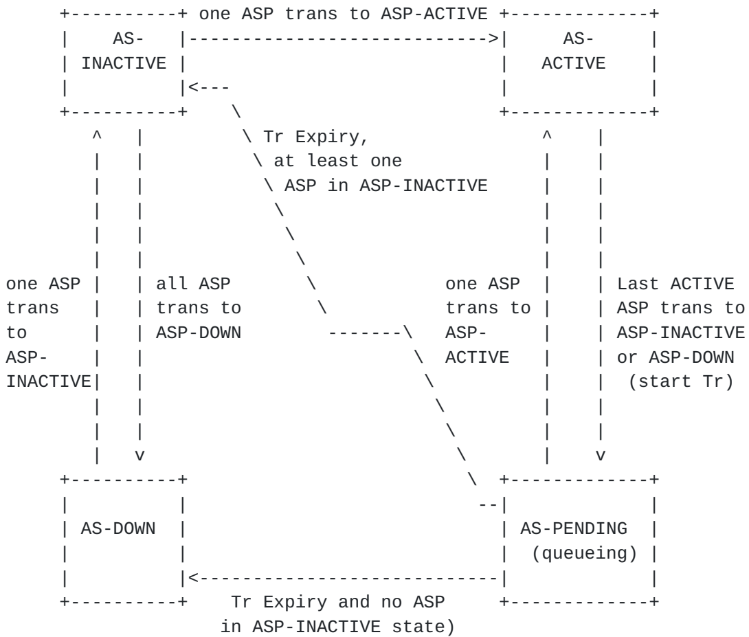
Figure 7: AS State Transition Diagram
