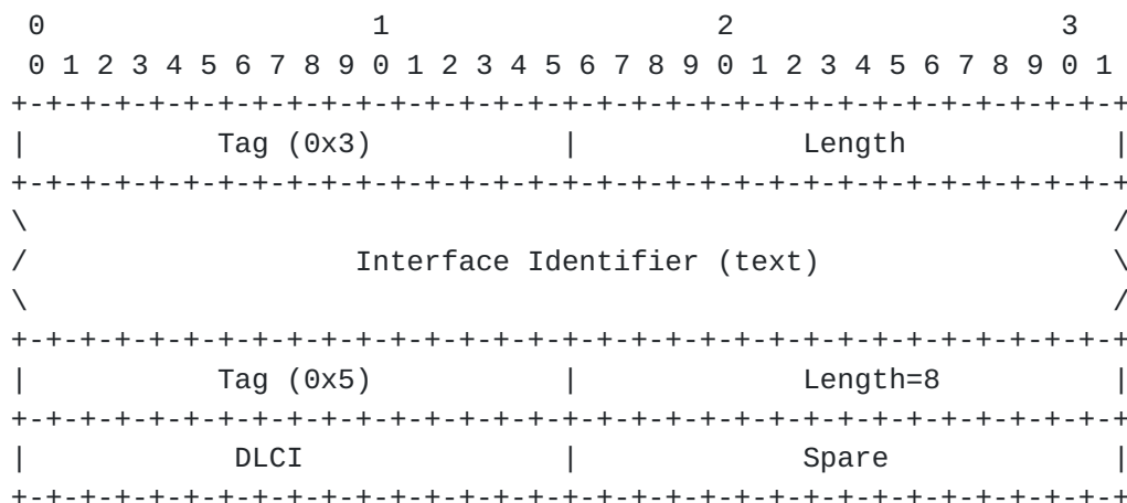
Figure 4 IUA Message Header (Text-based Interface Identifier)
