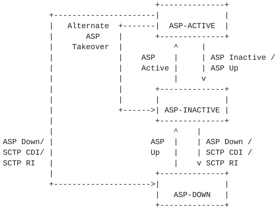
Figure 6 ASP State Transition Diagram
