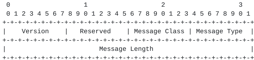
Figure 2 Common Header Format
