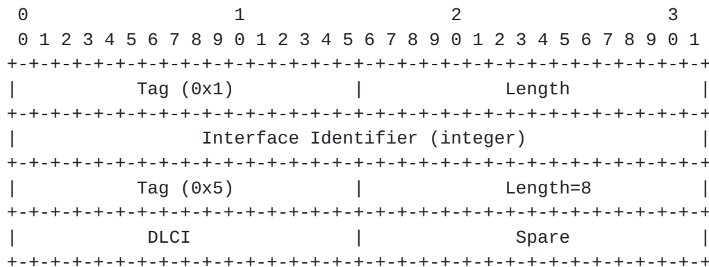
Figure 3 IUA Message Header (Integer-based Interface Identifier)
