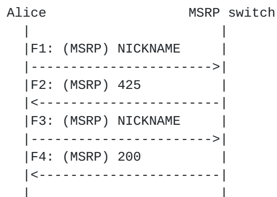
Figure 4: Flow diagram of a user setting up her nickname
