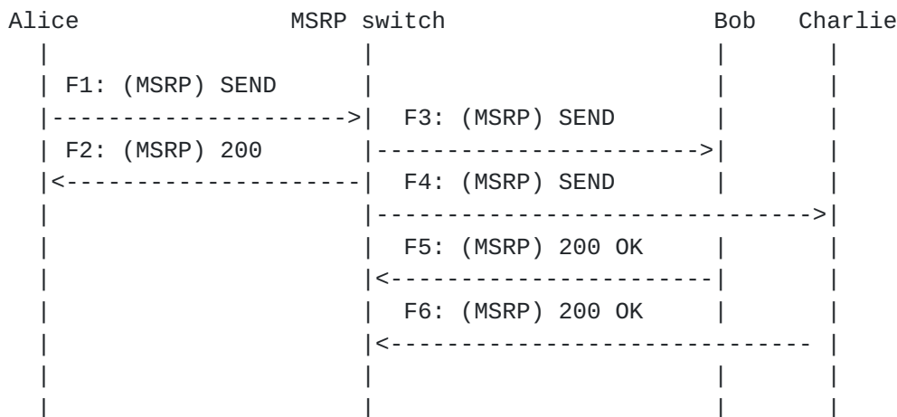
Figure 5: Sending a regular message to the chat room
