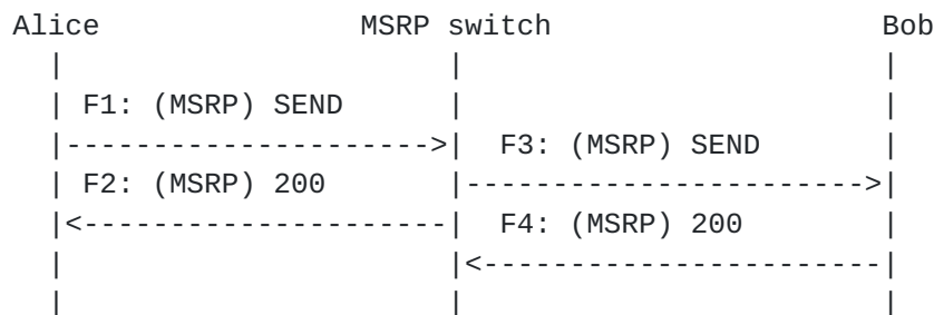
Figure 6: Sending a private message to Bob
