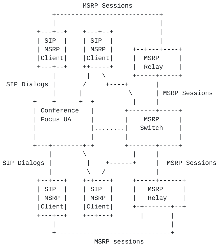
Figure 1: Multi-party chat overview shown with MSRP Relays and a conference Focus UA
