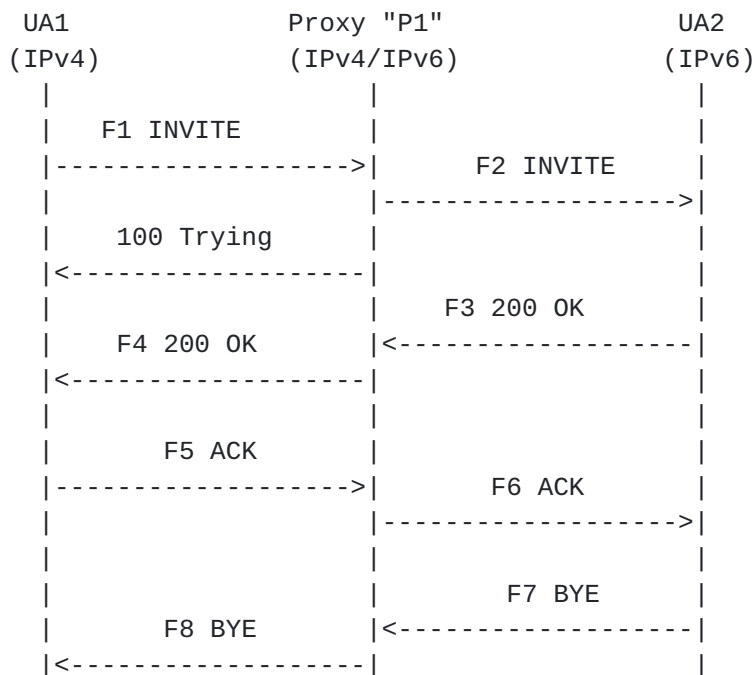
Figure 2: IPv4 to IPv6 multi-homed proxy illustration
