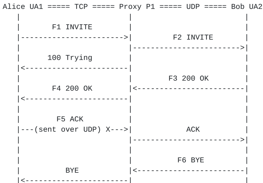
Figure 4: TCP to UDP transport protocol switching issue illustration
