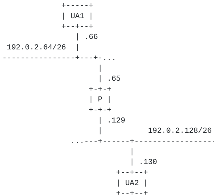
Figure 1: multi-homed proxy illustration
