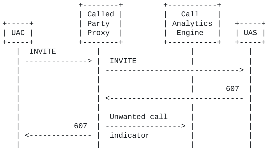
Figure 2: Unwanted (607) Ladder Diagram
