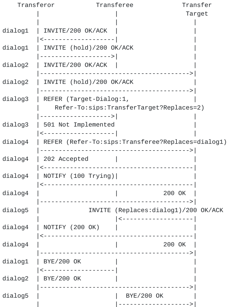
Figure 8. Recovery when one party does not support REFER.
