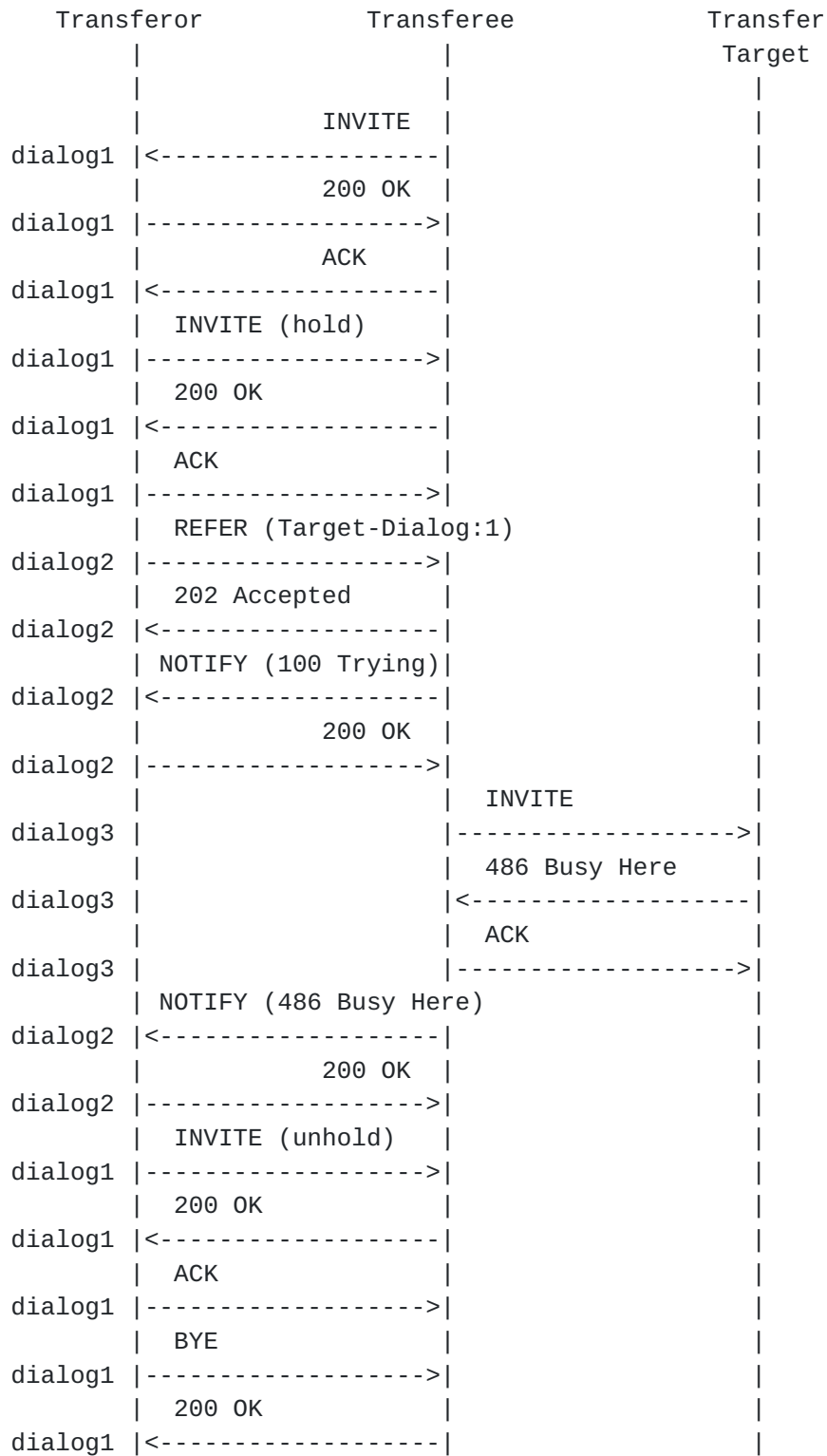
Figure 3. Failed Transfer - Target Busy
