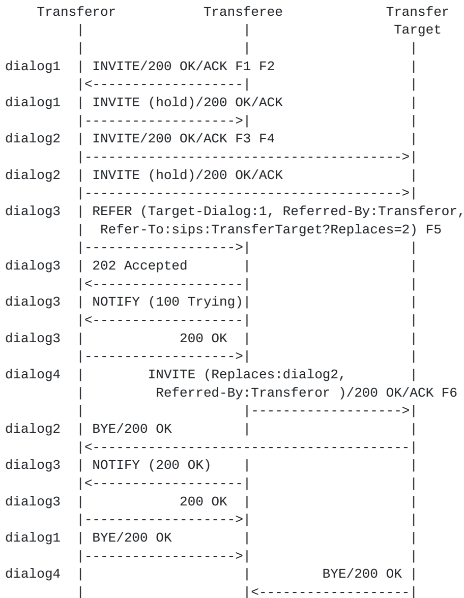
Figure 16. Attended Transfer Call Flow with Referred-By.
