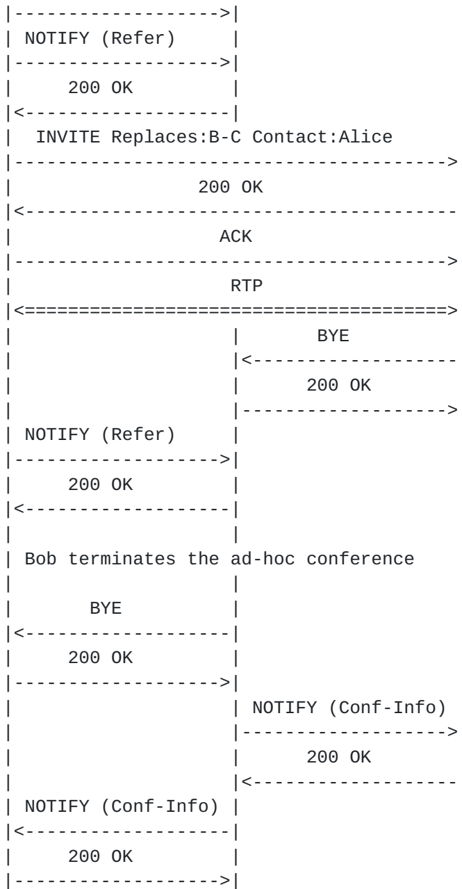
Figure 17. Attended Transfer as an Ad-Hoc Conference.
