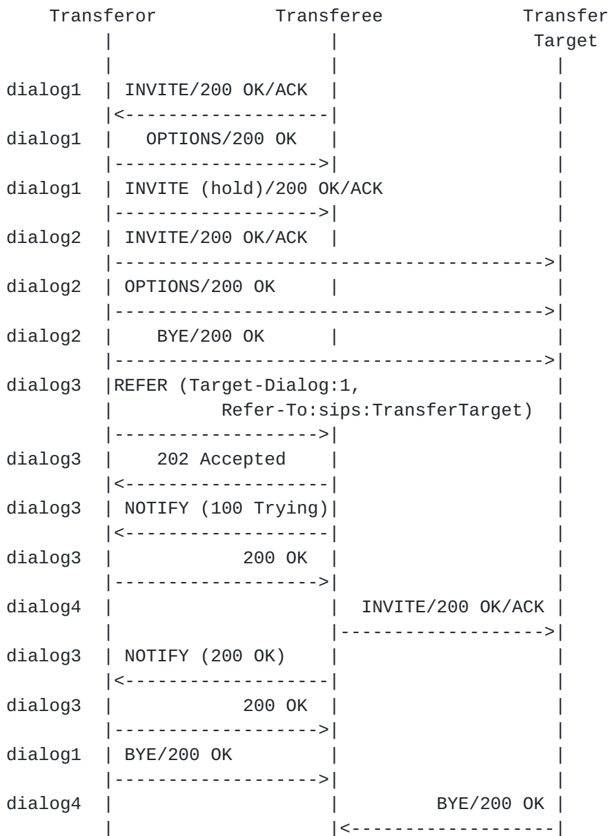
Figure 15. Attended Transfer Fallback to Basic Transfer.
