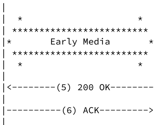
Figure 1: Message flow
