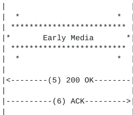
Figure 1: Message flow
