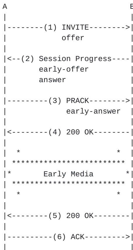
Figure 1: Message flow
