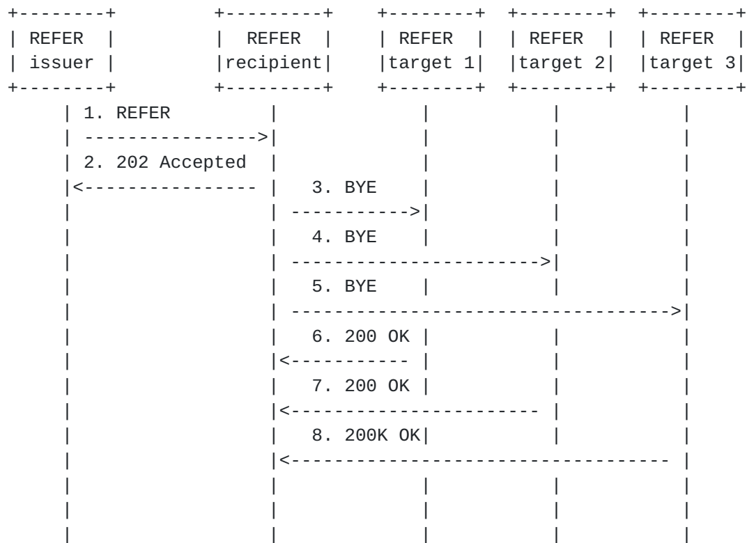
Figure 2: Example flow of a REFER request containing multiple REFER-Targets
