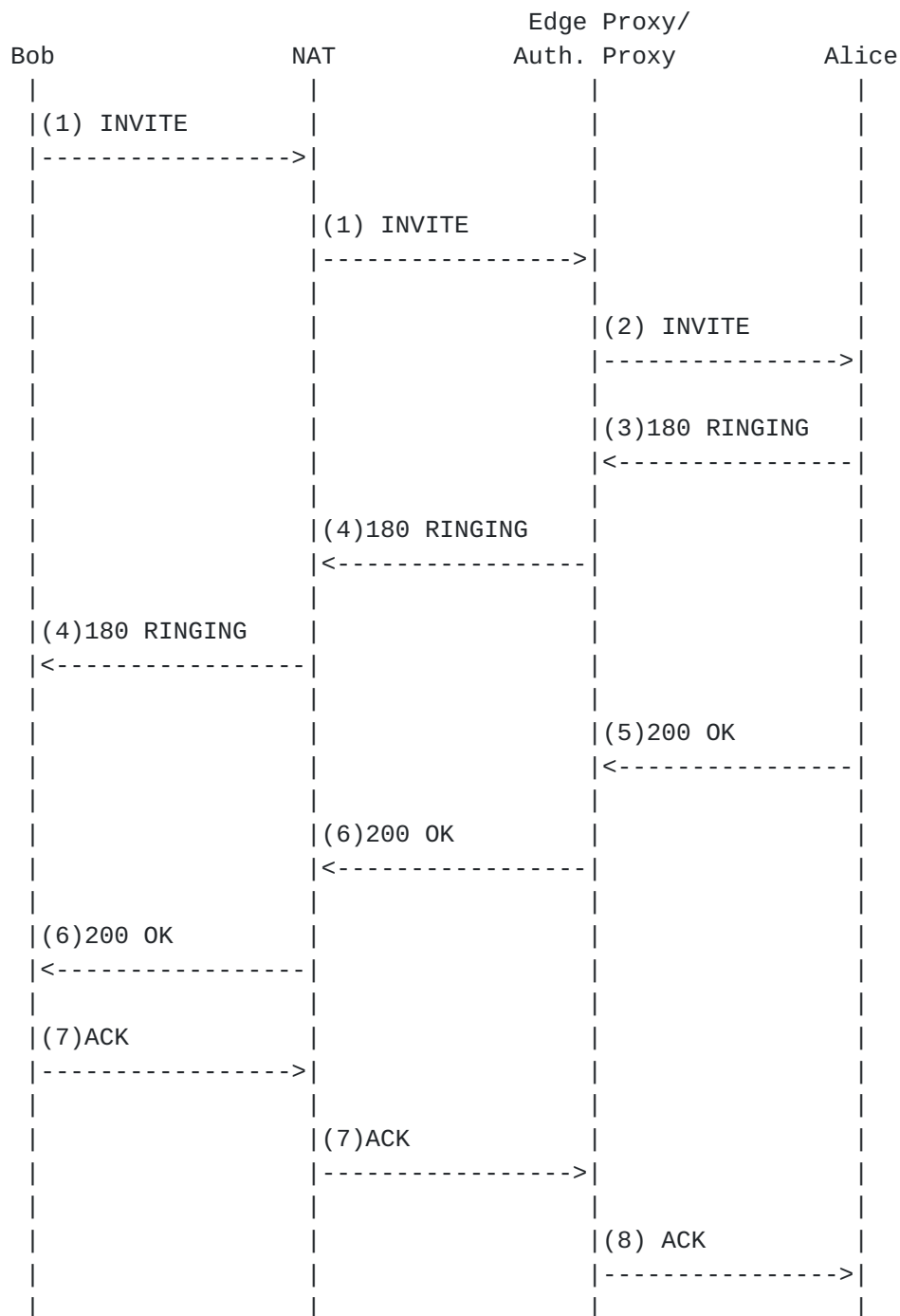
Figure 8: Initiating a Session - UDP
