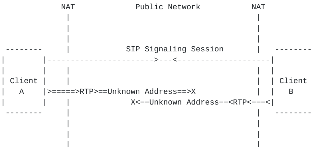
Figure 3: Failed Media
