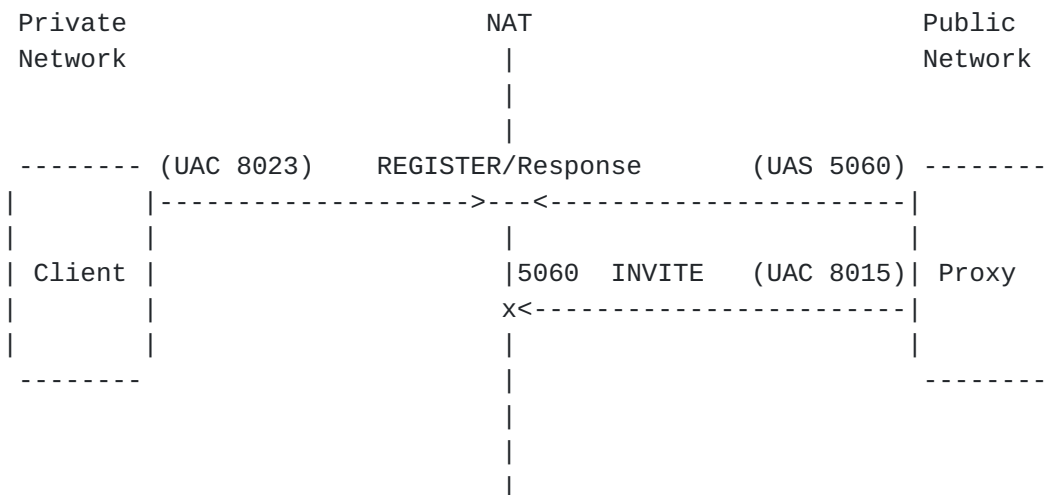
Figure 2: Failed Request
