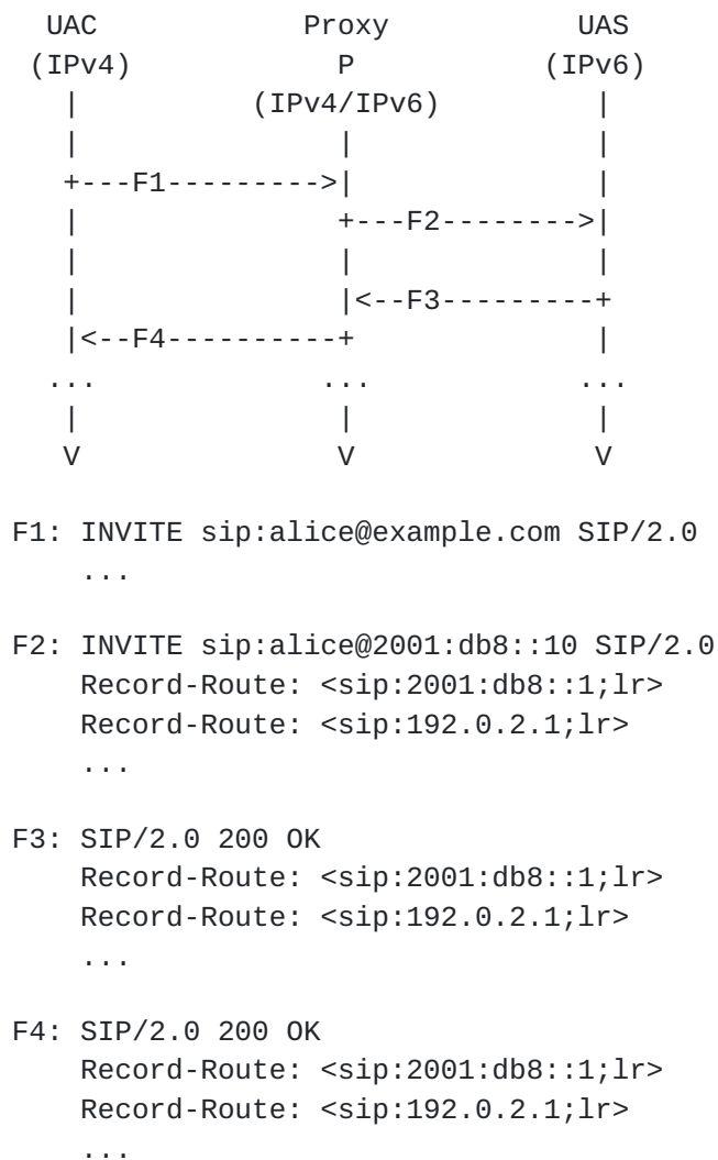
Figure 1: Relaying requests across different networks.
