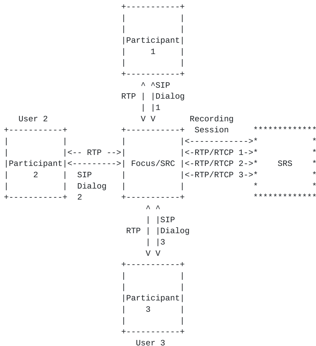
Figure 5: Conference Focus acting as an SRC.
