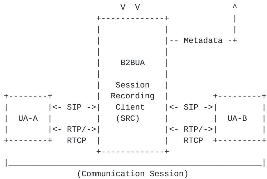
Figure 1: B2BUA Acts as the Session Recording Client.
