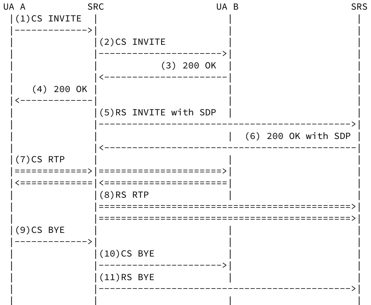
Figure 1: Basic recording call flow
