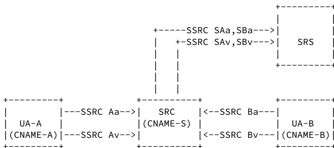
Figure 10: SRC Using SSRC Multiplexing
