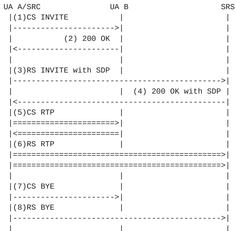
Figure 1: Basic recording call flow with UA as SRC
