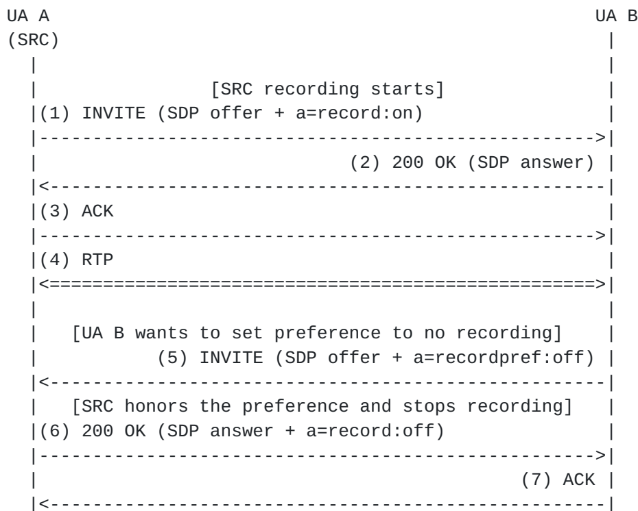
Figure 4: Recording indication and recording preference
