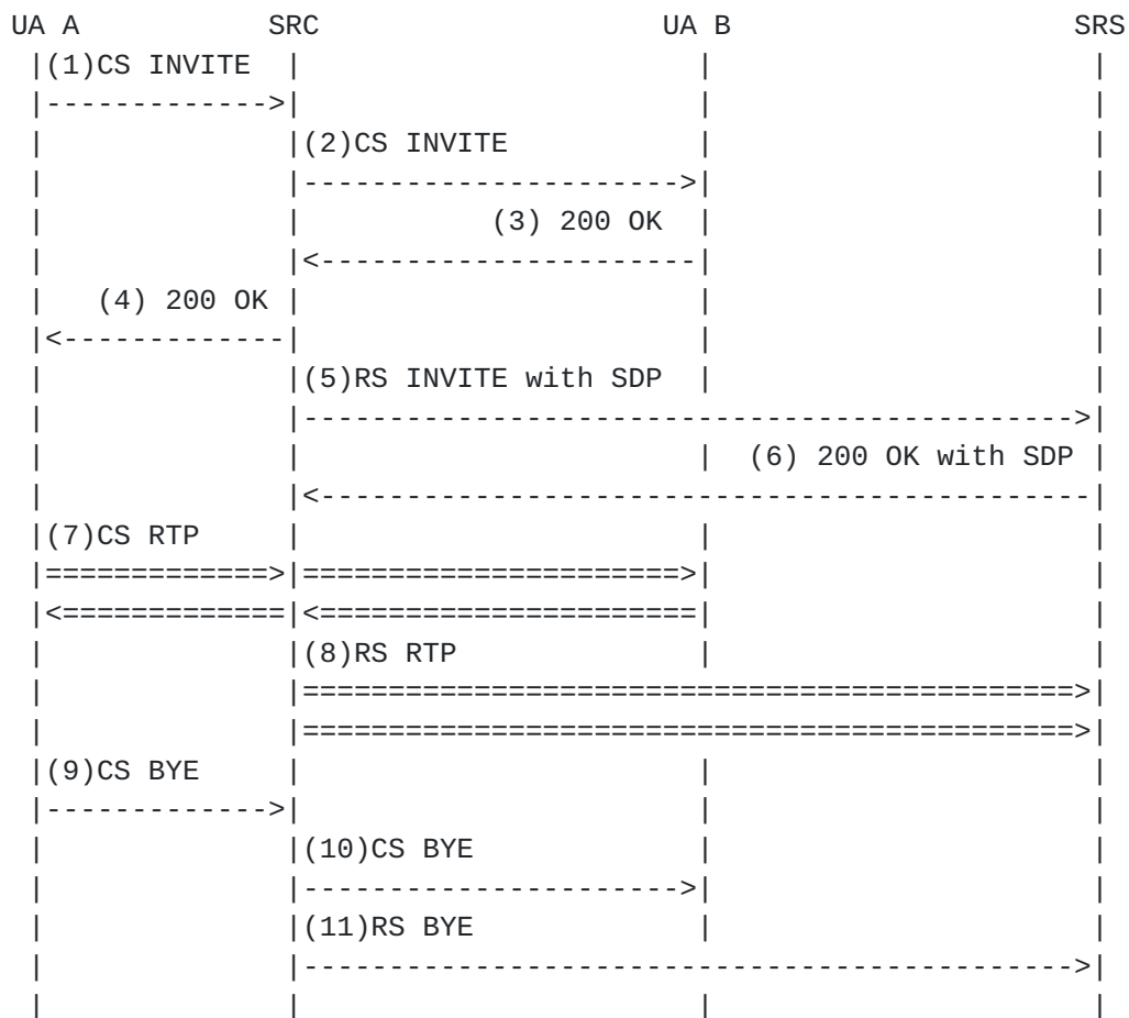
Figure 2: Basic recording call flow with B2BUA as SRC
