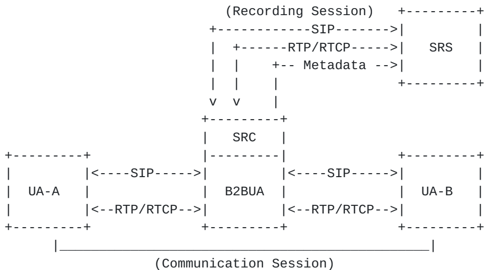
Figure 9: B2BUA as SRC
