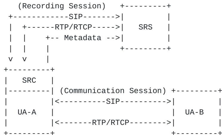
Figure 8: UA as SRC
