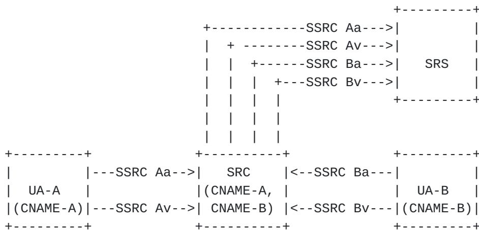
Figure 10: SRC Using Multiple m-lines
