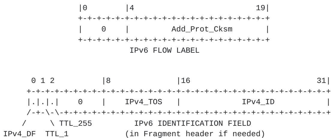
4rd Identification fields of IPv6 Fragment headers
