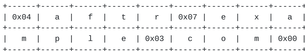
Figure 2: Example tunnel-endpoint-name.
