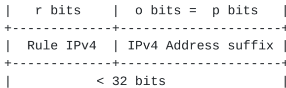
Figure 4: IPv4 prefix
