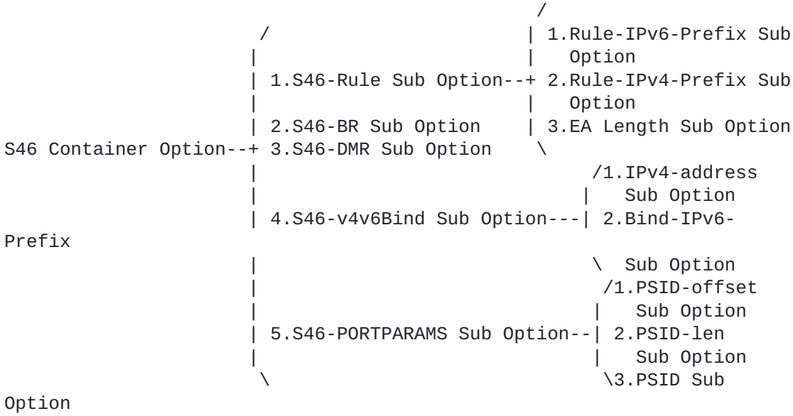
Figure 2: S46 Container Option Hierarchy
