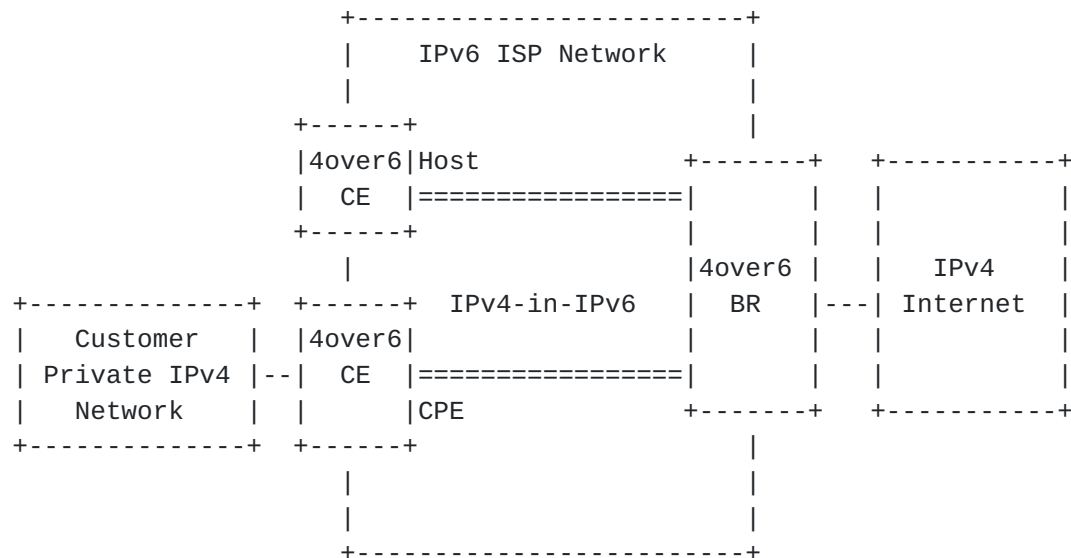
Figure 1 Public 4over6 scenario
