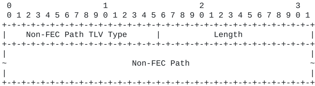
Figure 1: Non-FEC Path TLV Format
