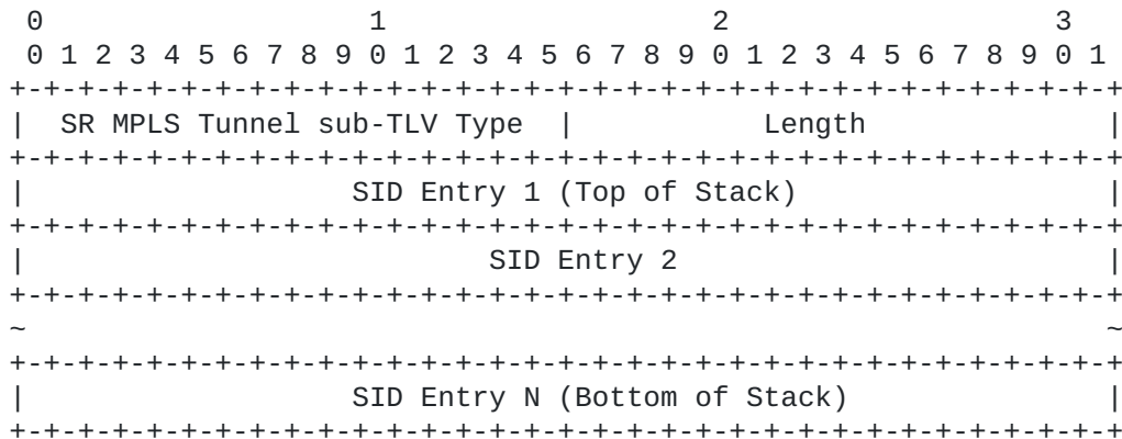
Figure 2: Segment Routing MPLS Tunnel sub-TLV
