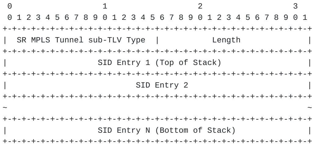
Figure 2: Segment Routing MPLS Tunnel sub-TLV
