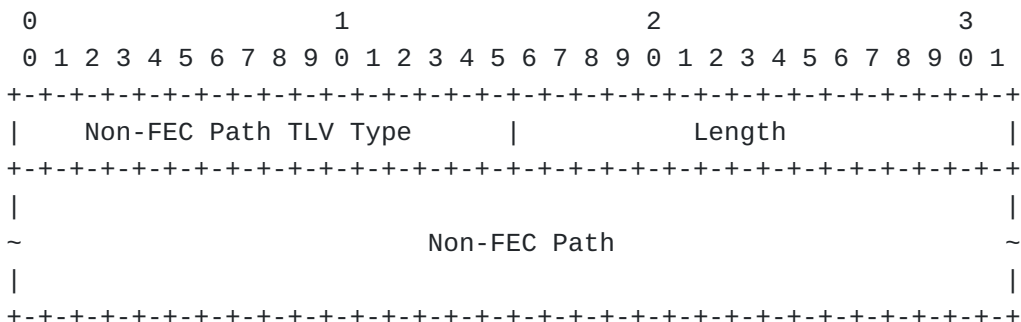
Figure 1: Non-FEC Path TLV Format
