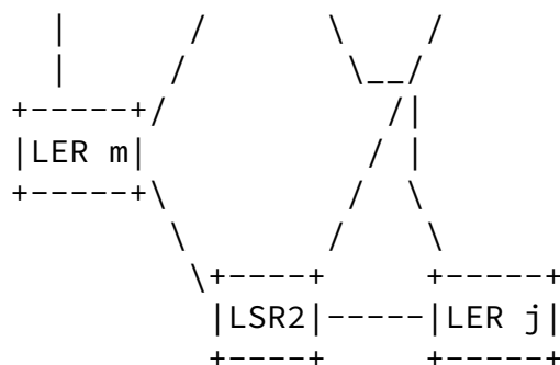
Example of a PMS based LSP dataplane monitoring
