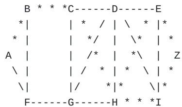
Figure 3: Reference topology
