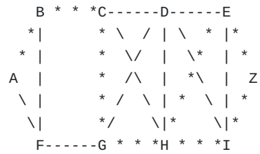
Figure 5: Managed shortest path protection
