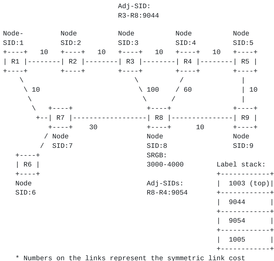
Figure 3: Explicit path using an Adj-SID. All nodes have SRGB = [1000-2000], except for R8 which has SRGB = [3000-4000].
