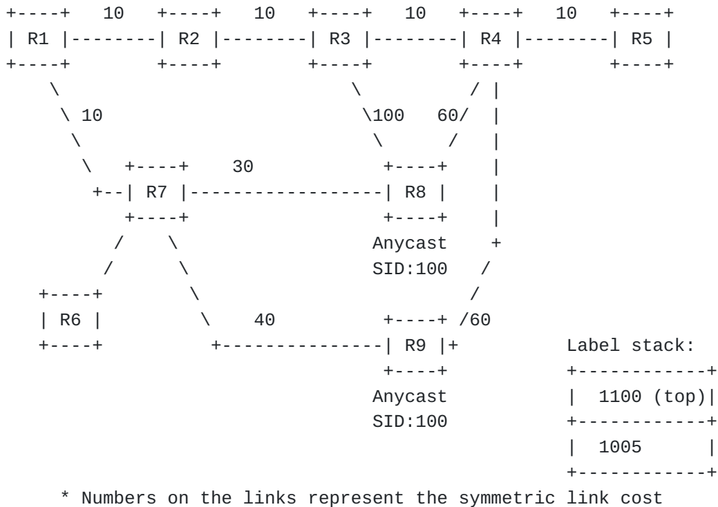
Figure 2: Topology illustrating use of Anycast-SIDs to protect against node failures. All nodes have SRGB = [1000-2000].
