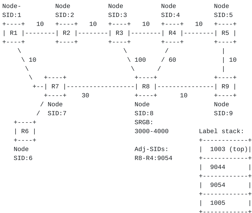
Figure 3: Explicit path using an Adj-SID. All nodes have SRGB = [1000-2000], except for R8 which has SRGB = [3000-4000].
