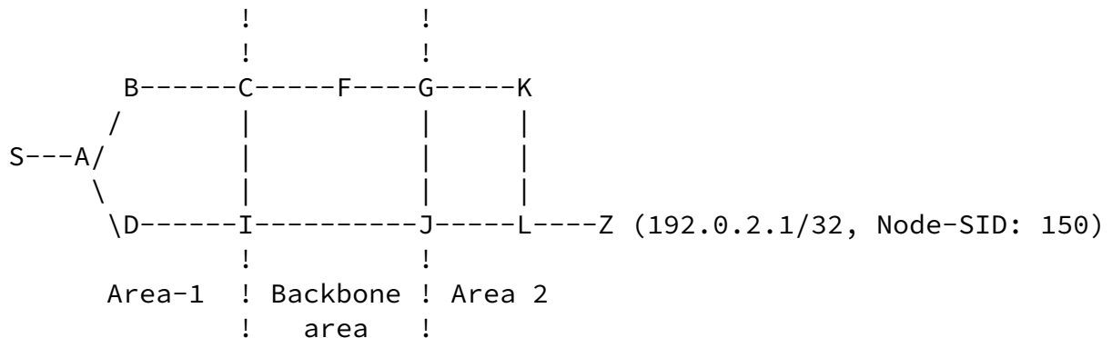
Figure 1: Inter-Area Topology Example
