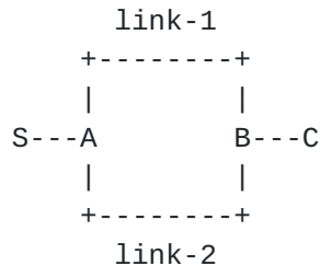
Figure 1: Parallel Links and Adj-SIDs
