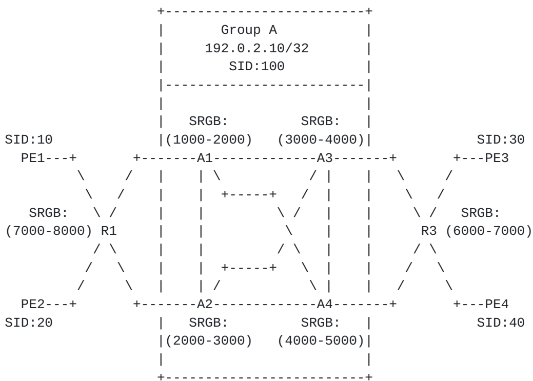
Transit paths via anycast group A
