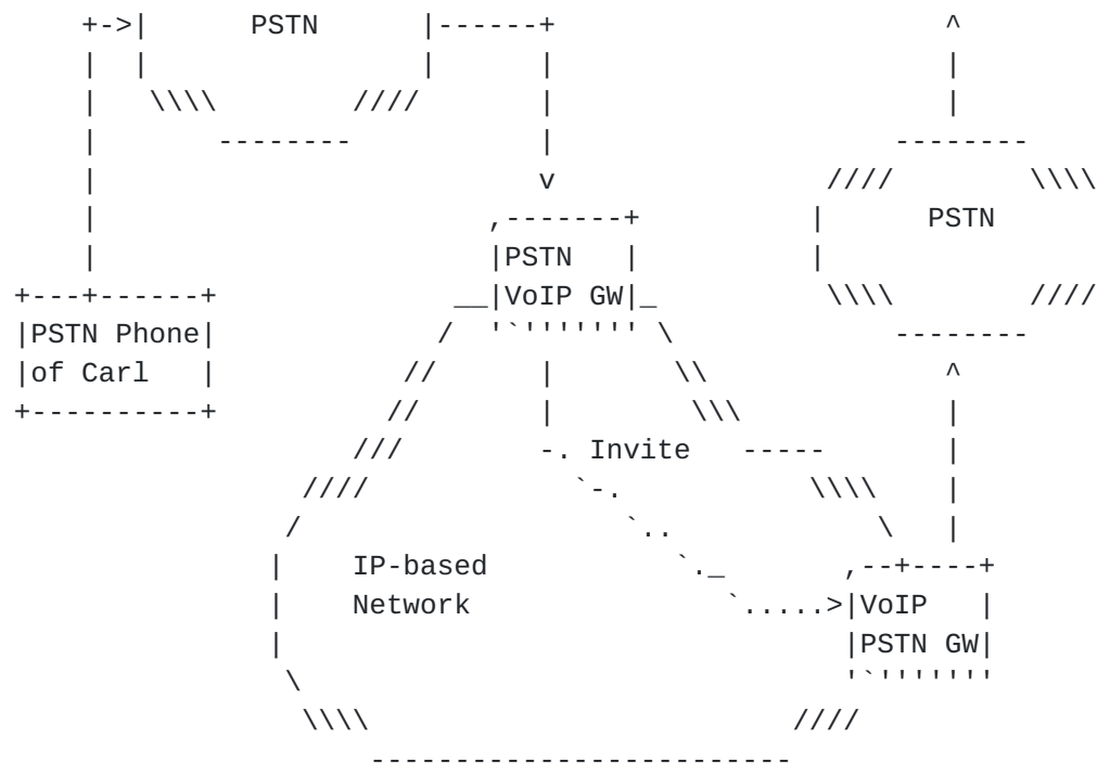
Figure 5: PSTN-VoIP-PSTN Call.
