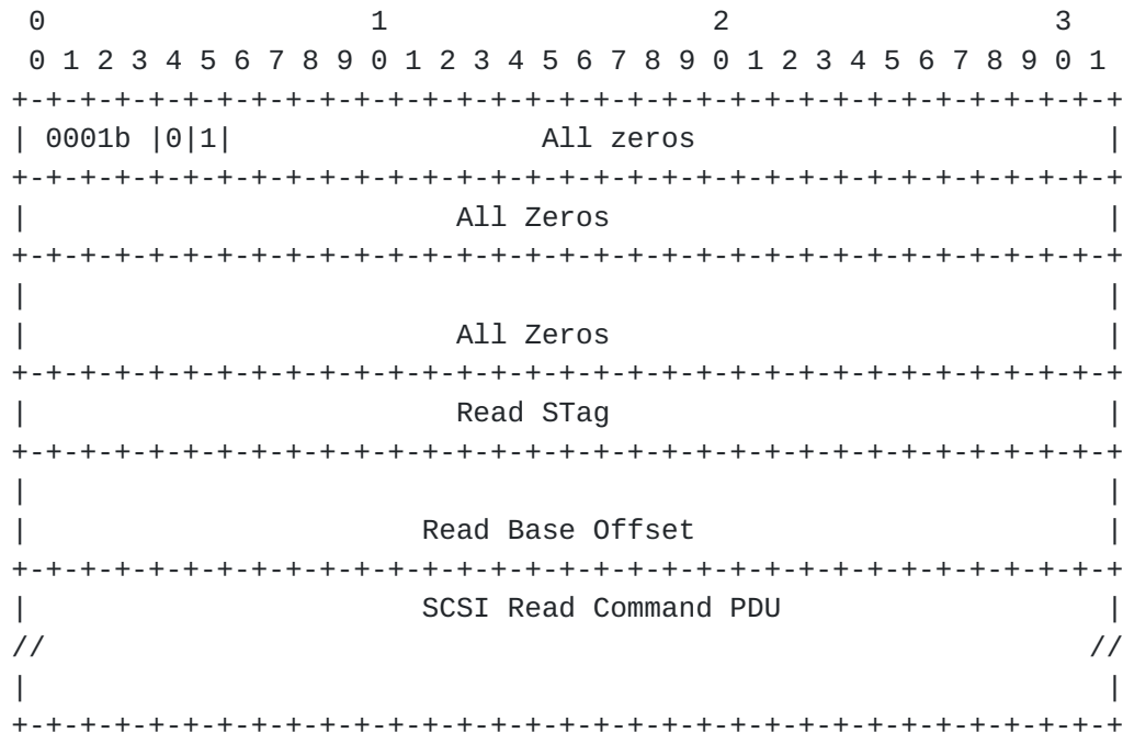
Figure 8 iSER Header Format for SCSI Read Command PDU
