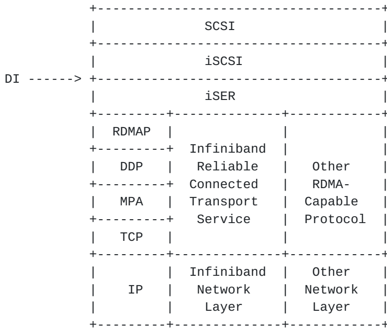
Figure 1 Example of iSCSI/iSER Layering in Full Feature Phase
