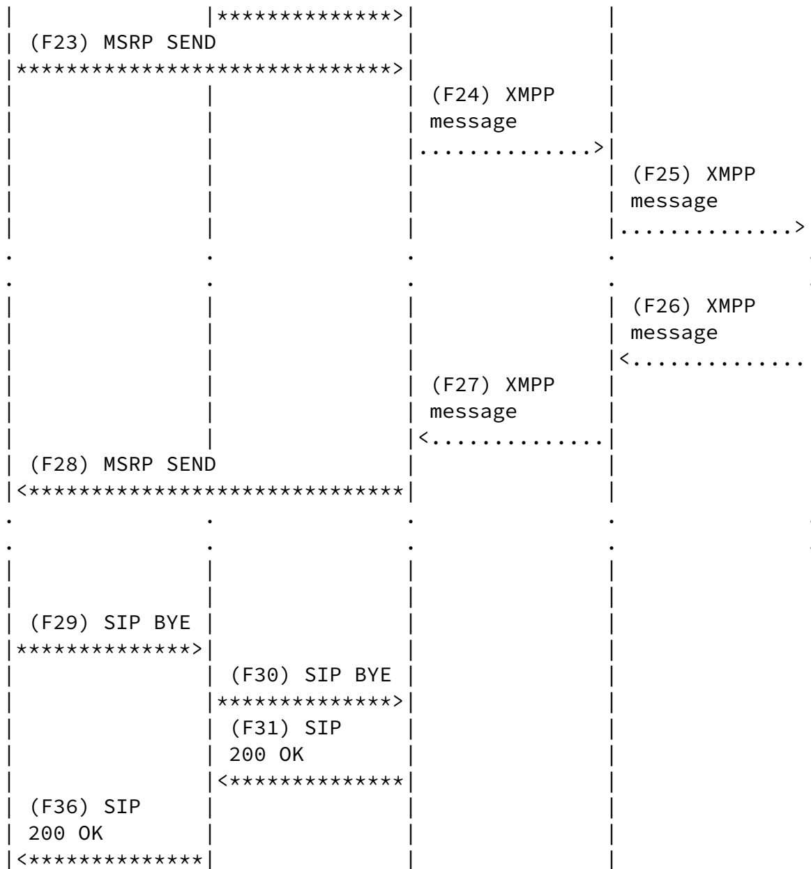
Figure 2: MSRP to XMPP Order of Events
