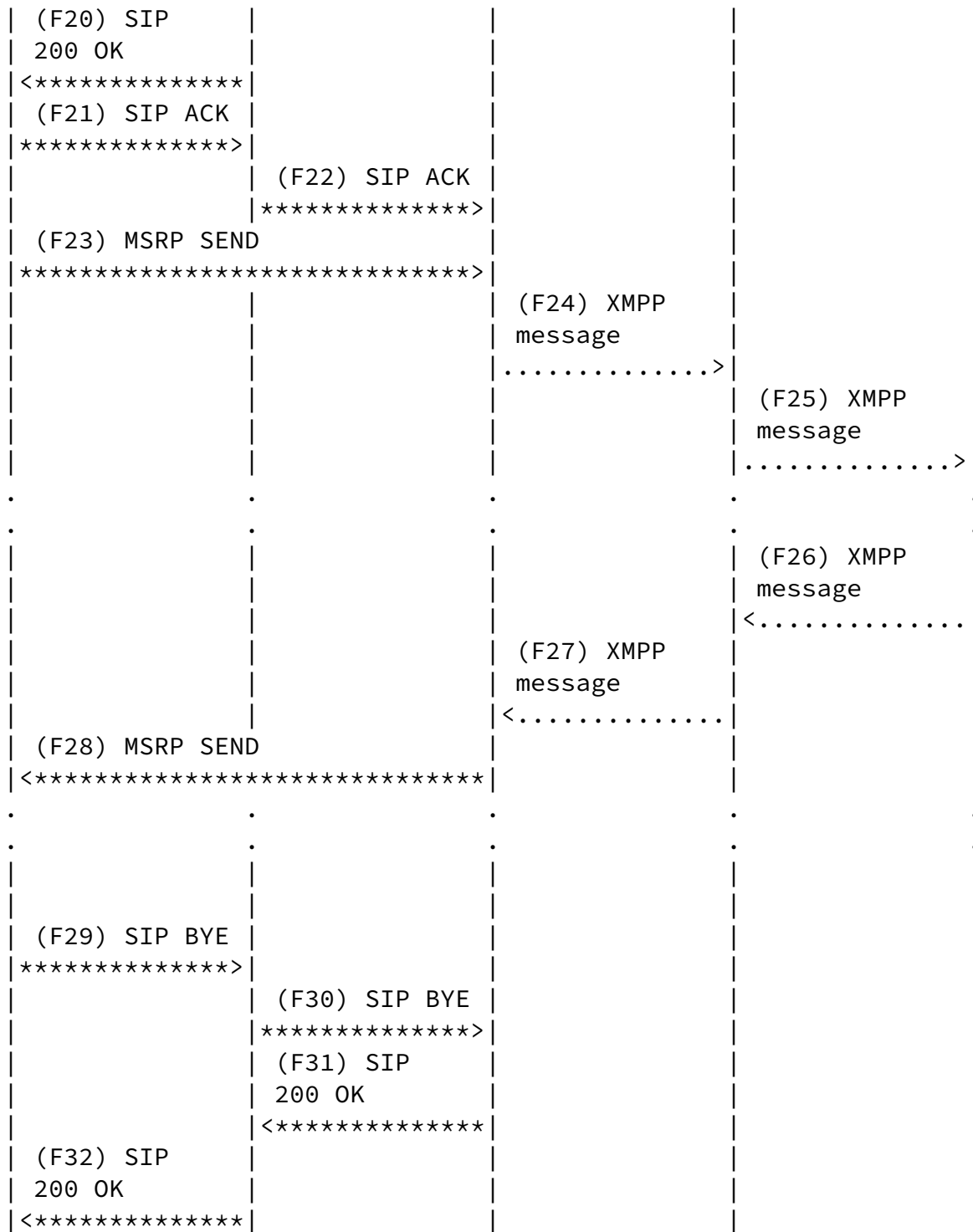
Figure 2: MSRP to XMPP Order of Events
