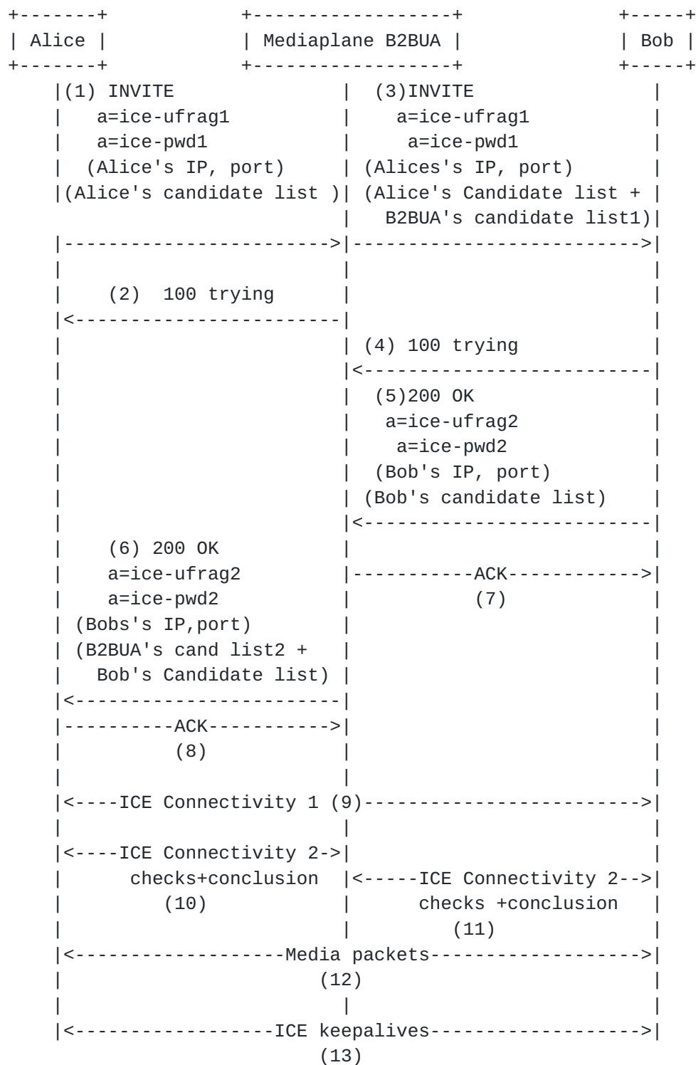
Figure 2: INVITE with SDP having ICE and with a Media Plane B2BUA in optional ICE termination mode
