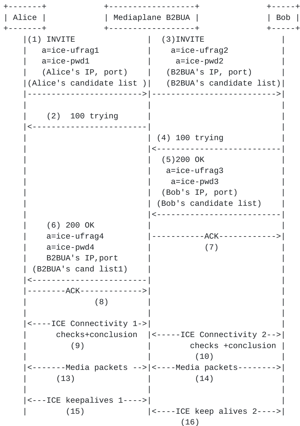
Figure 1: INVITE with SDP having ICE and with a Media Plane B2BUA terminating ICE
