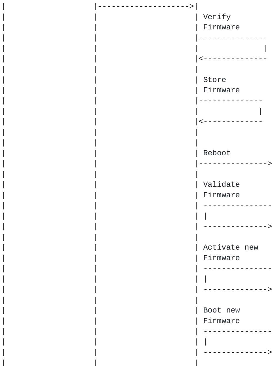
Figure 5: Example Flow for a Firmware Upate.
