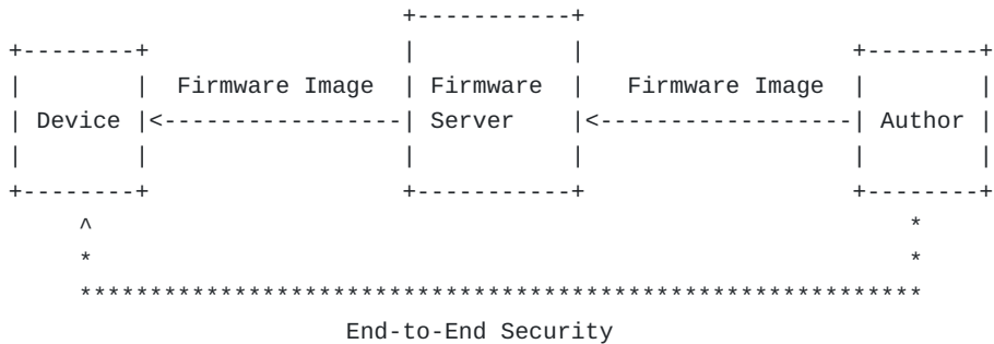
Figure 2: End-to-End Security.
