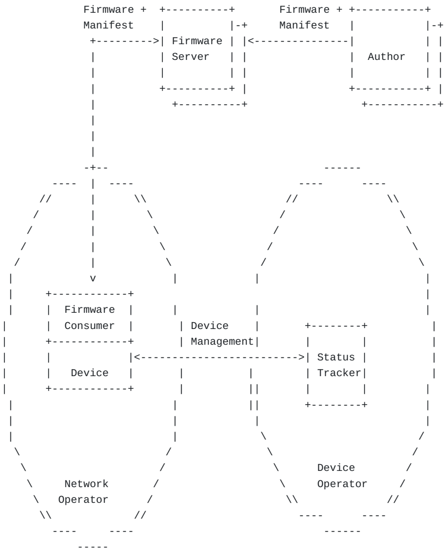
Figure 1: Architecture.
