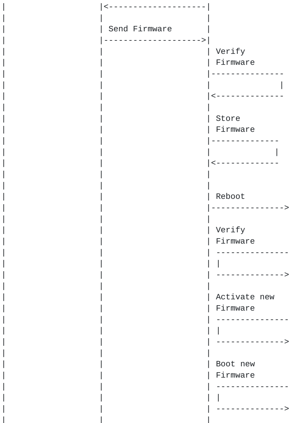
Figure 5: Example Flow for a Firmware Update.
