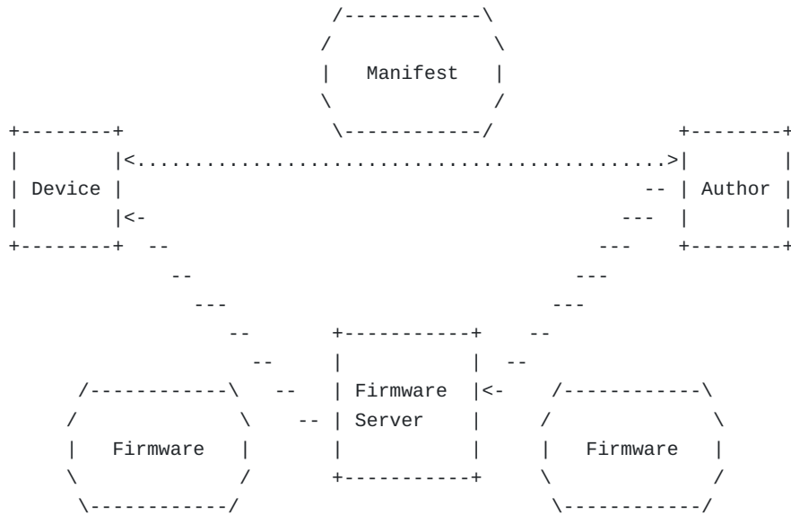
Figure 4: Independent retrieval of the firmware image.
