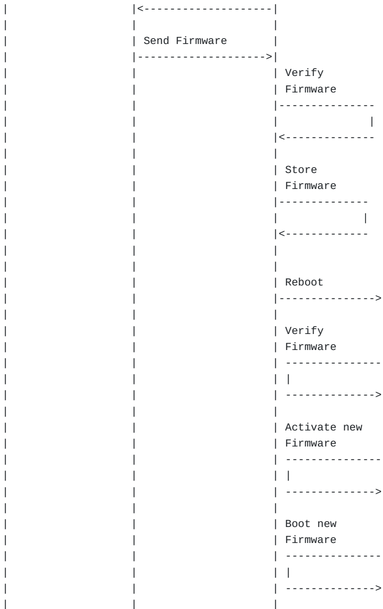
Figure 5: Example Flow for a Firmware Update.
