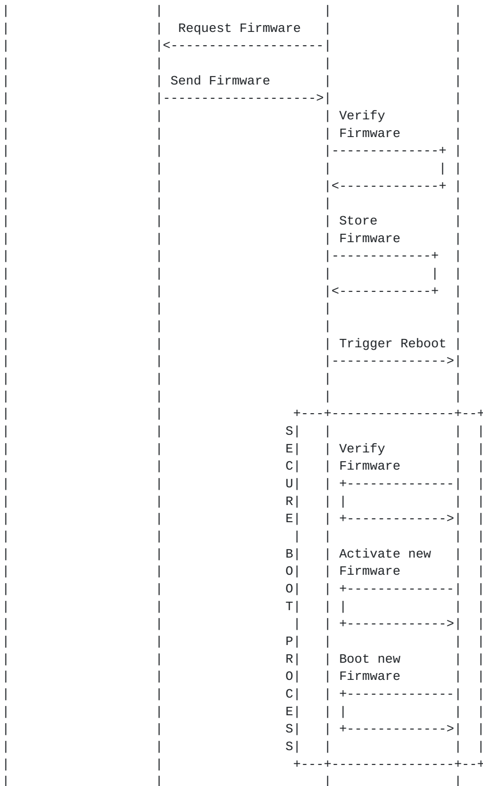
Figure 5: First Example Flow for a Firmware Upate.
