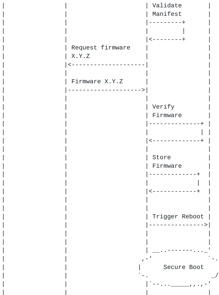
Figure 6: Second Example Flow for a Firmware Upate.
