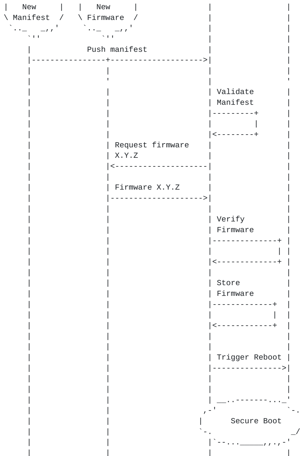
Figure 6: Second Example Flow for a Firmware Upate.
