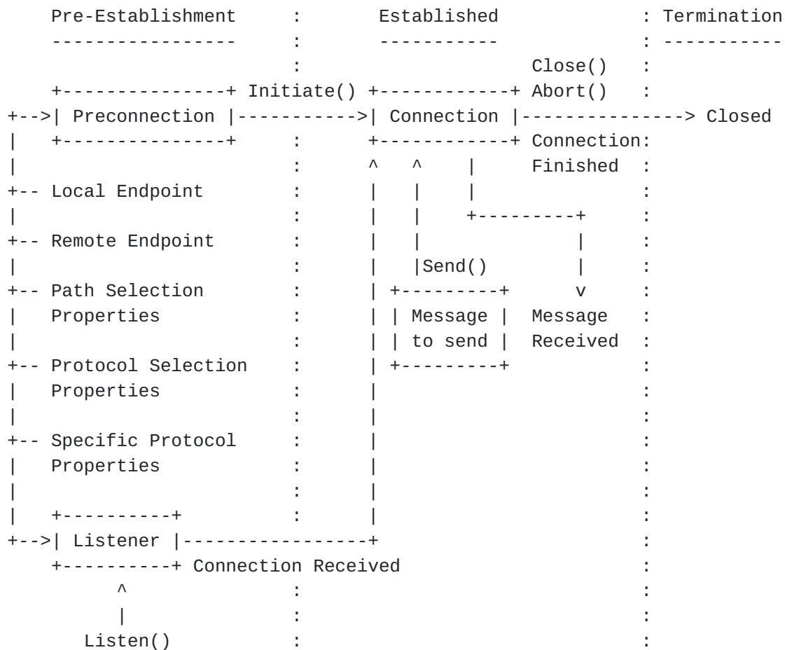
Figure 2: The lifetime of a connection
