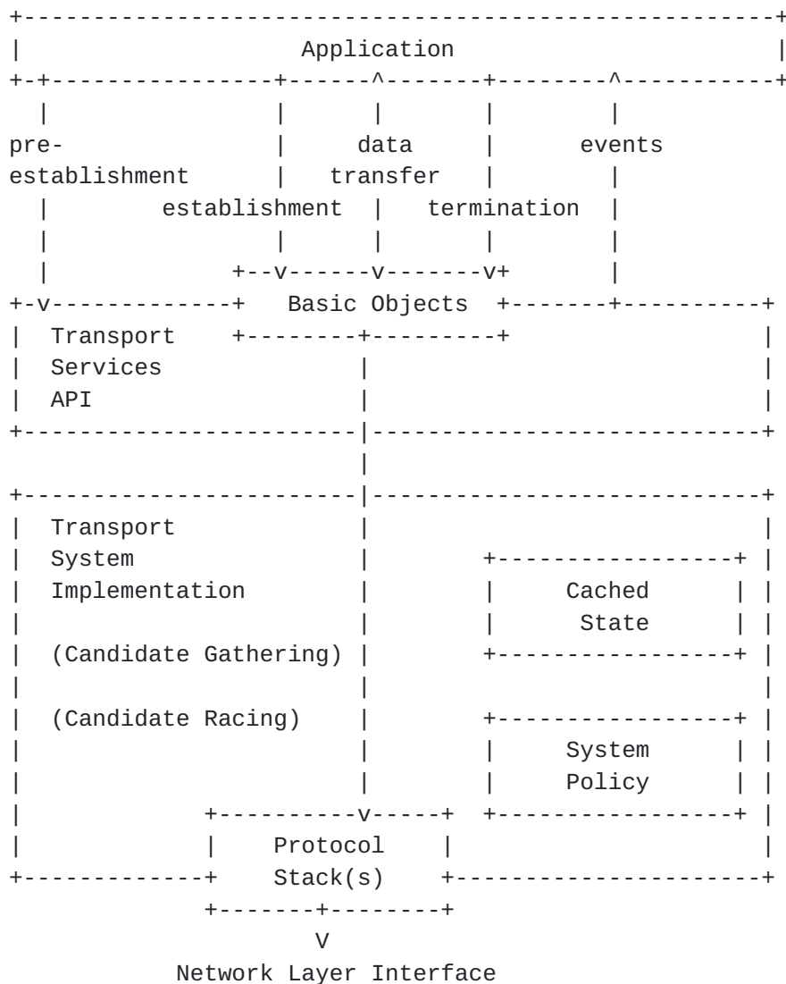
Figure 1: Concepts and Relationships in the Transport Services Architecture
